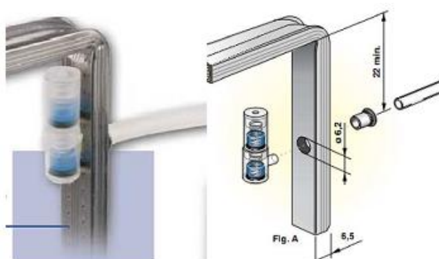
Fig.12 Installation of two-way pressure valve into glass unit
