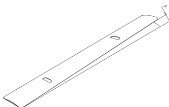
Fig. 17 Deviation of slat parallel from horizontal
