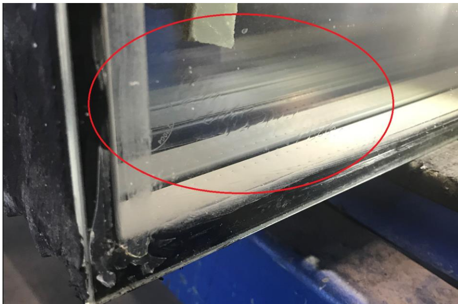
Fig. 35 Delamination of PVB film due to chemical incompatibility
