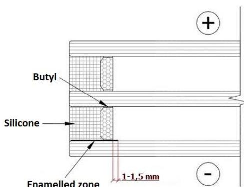
Fig. 27 Enamel zone for insulating glass units intended for bonded glazing
