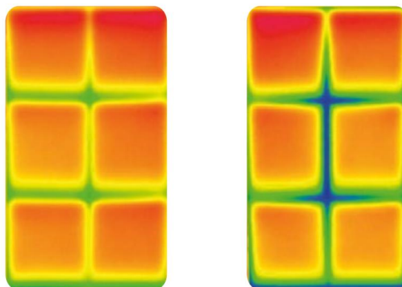
Fig. 33 On the left, the cold bridge with a "warm" insert, on the right with an aluminum insert
