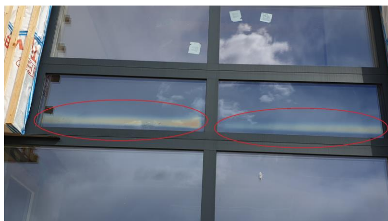
Fig. 36 Chemical evaporation inside the insulating glass unit after exceeding recommended temperature of 60 °C
