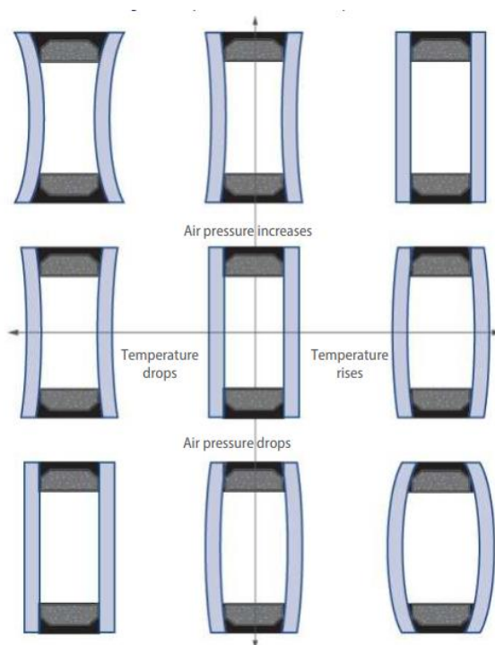
Fig. 28 Concavity/convexity of glasses, depending on temperature and atmospheric pressure
