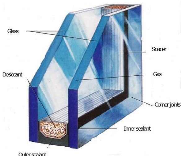
Fig. 1 Standard structure of double-glazed insulating glass units
