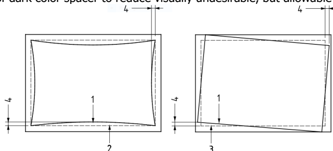
Fig. 8 Examples of spacer deviation
