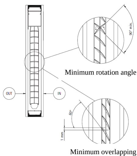
Fig. 21 Overlapping of slats
