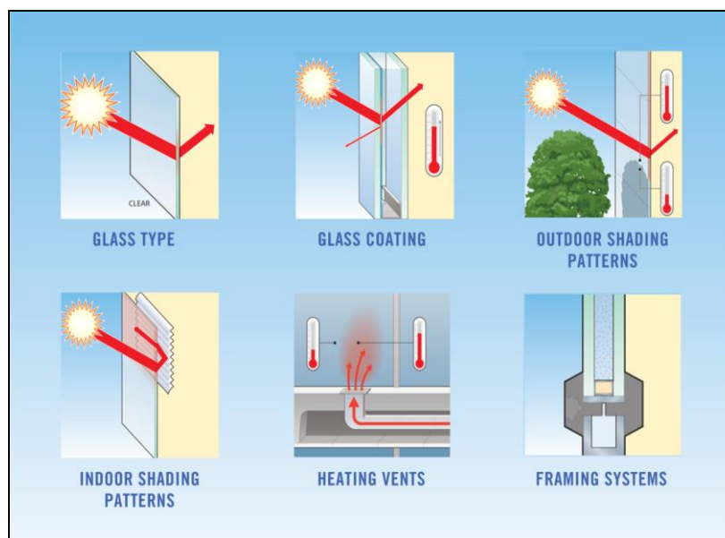
Fig. 37 Factors having influence on the risk of thermal breakage
