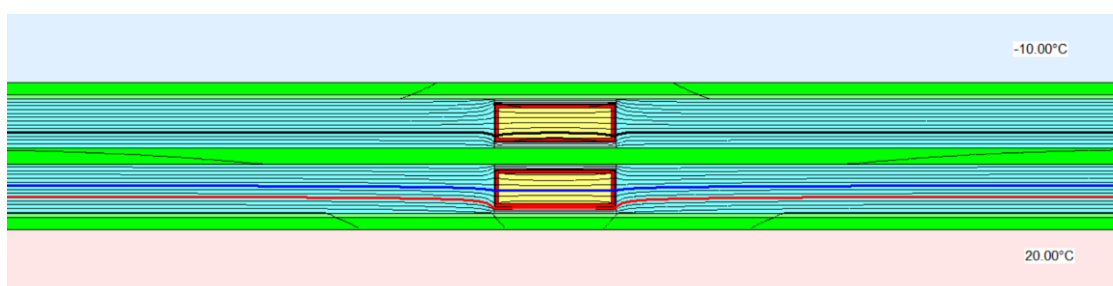
Fig. 32 The linear thermal transmittance, when minimum surface temperature with -10° C externally (black 0° C, blue 10° C, red 13° C isothermal lines)
