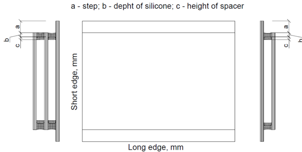
Fig. 3 Drawing of a structural glazing unit
