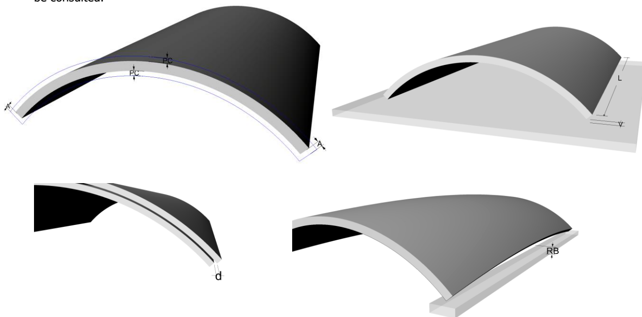
Fig. 22 Deviation of bended glazing Allowable deviation of bended glasses
